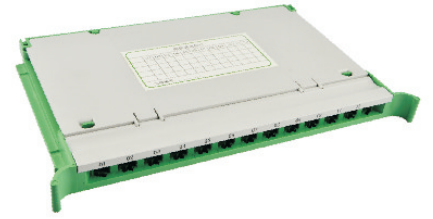
PartNumber Dimension(A*B*C) FOST-12C 302*195*25(mm)
