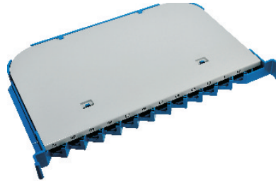
PartNumber Dimension(A*B*C) FOST-12B 320*215*25(mm)
